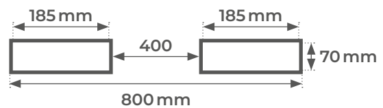
DGG2 CLAMP FOR TWO BARRELS
