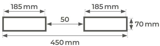
DGG1 CLAMP FOR ONE BARREL
