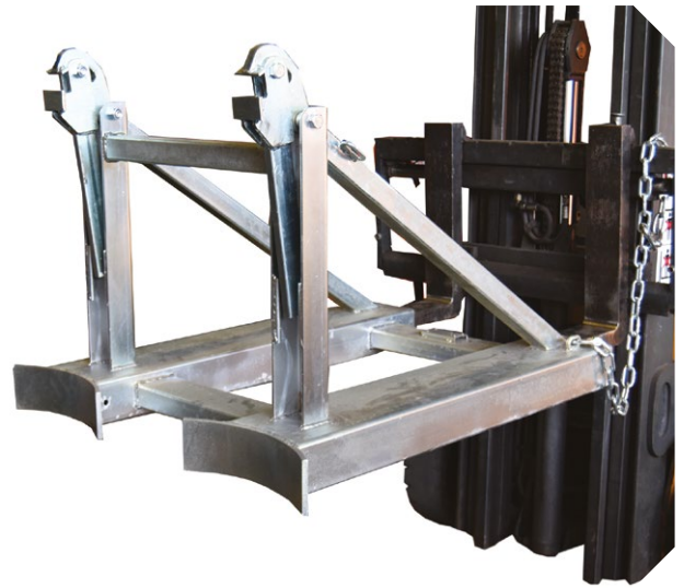
DGG2 CLAMP FOR TWO BARRELS
